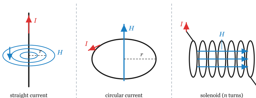
Figure 4-1-3 · Three geometries: the field circles a straight current, threads the center of a circular current, and runs uniform inside a solenoid.
