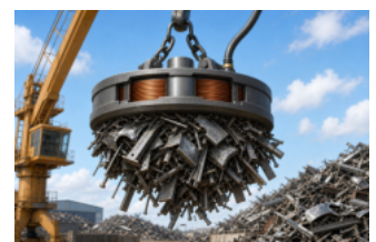
Figure 4-1-7 · A scrap-yard lifting electromagnet — a coil of many copper turns wound on an iron core, fed by an insulated power cable — grips a dense clump of steel scrap beneath its flat face and holds it against gravity, with only ferromagnetic material clinging on, densest at the face.
