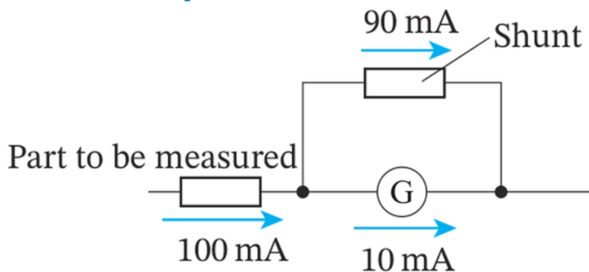
Figure 3-1-6 · Worked Example (a): a shunt beside the galvanometer G carries 90 mA of the 100 mA line current, so the needle still reads only its 10 mA full-scale value.
