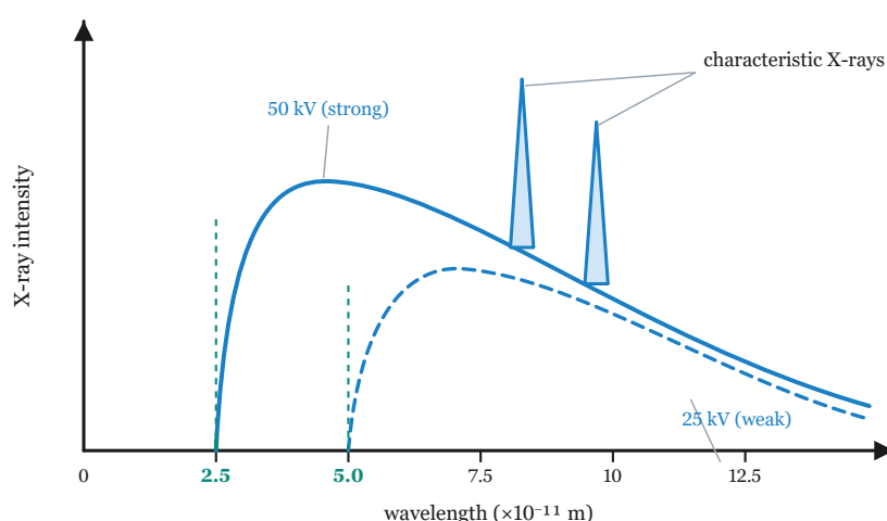
Figure 5-2-2 · Two measured X-ray spectra from the same metal target: the solid curve at 50 kV cuts off at 2.5 \times 10^{-11} m, the dashed curve at 25 kV at 5.0 \times 10^{-11} m. The characteristic peaks sit at wavelengths fixed by the metal, so they do not move with the voltage.
