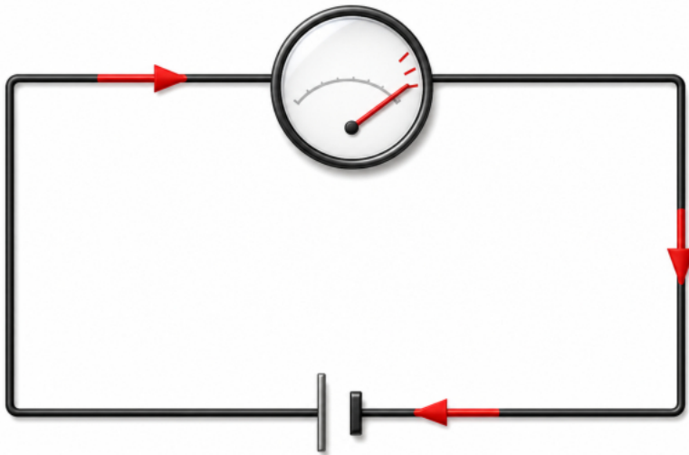
Figure 3-1-1 · A single bare galvanometer movement rated for only 10 mA is placed directly in a branch carrying 200 mA, so its needle is driven far past full scale.
