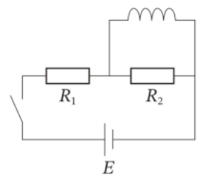
Figure 4-5-6 · Try 1: the battery \varepsilon , the resistors R_1 and R_2 , the coil, and the switch, connected as described.
