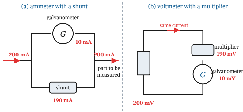
Figure 3-1-3 · The two arrangements set side by side, so the mirror symmetry between them can be read off in one glance: on the left the added resistor sits beside the movement, which forces the two to share a voltage and lets them divide a current; on the right it sits ahead of the movement, which forces them to share a current and lets them divide a voltage. Each design condition is simply the property of its own connection — that is the reasoning the Point's two figures leave implicit.
