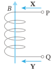
Figure 4-4-6 · Try: the coil with terminals P and Q, the reference arrow B fixing the positive direction, and the two senses X and Y in the outside circuit.
