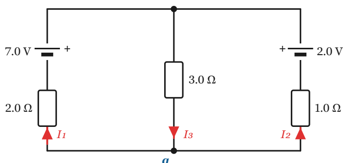
Figure 3-2-10 · Exercise 2: batteries 7.0 V and 2.0 V with resistors 2.0 \Omega , 3.0 \Omega , and 1.0 \Omega in a two-loop network — the 7.0 V battery shares its branch with the 2.0 \Omega resistor, the 2.0 V battery with the 1.0 \Omega resistor, and the 3.0 \Omega resistor is the shared middle branch.
