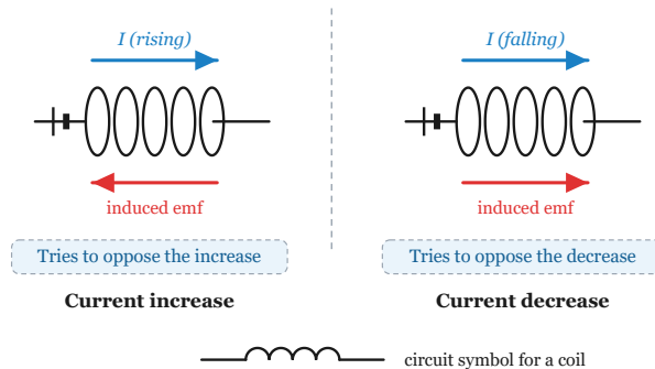
Figure 4-5-3 · When the current rises the coil induces an emf that opposes the increase; when it falls the coil induces an emf that opposes the decrease. Alongside is the circuit symbol for a coil.
