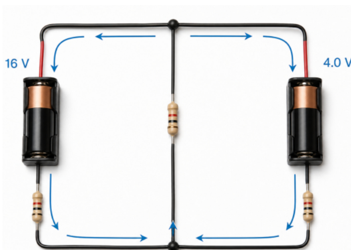
Figure 3-2-1 · Two batteries of unequal emf drive three resistors in two loops that share a middle branch and meet at a junction.
