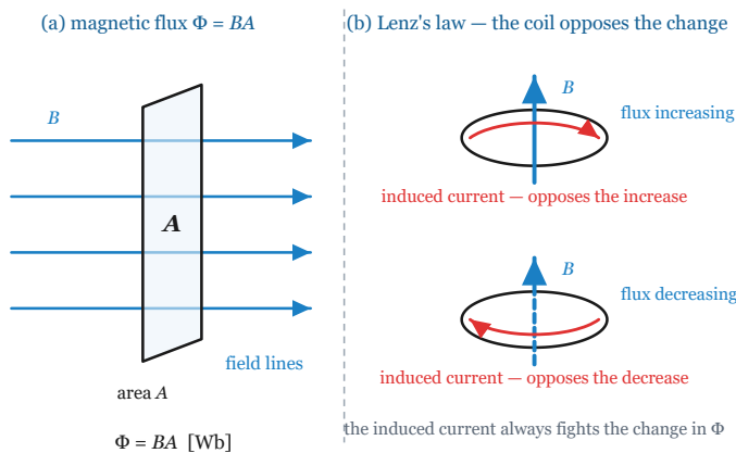
Figure 4-4-3 · Left: field lines of density B through an area A give the flux \Phi = BA . Right: by Lenz's law the induced current circulates so its own flux opposes the change — resisting an increase (top) and a decrease (bottom).
