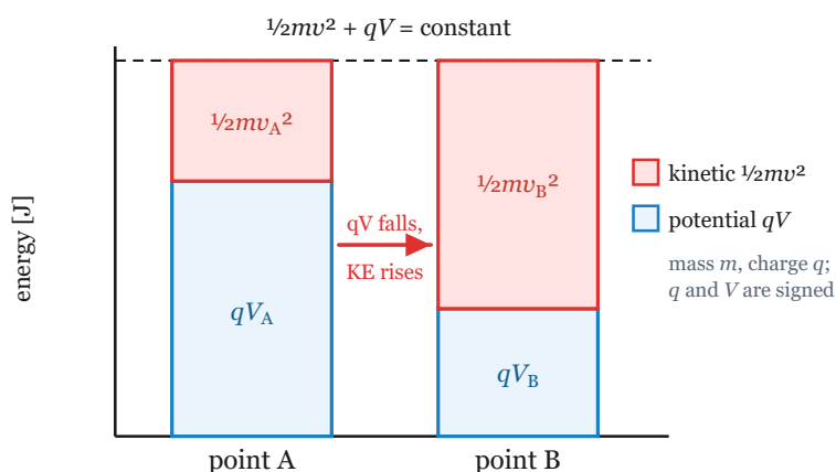
Figure 2-5-3 · Energy bars at points A and B: the electrostatic potential energy qV (blue) and the kinetic energy \frac{1}{2}mv^2 (red) trade places, but their sum reaches the same constant total at both points, so as qV falls from A to B the kinetic energy rises by the same amount.
