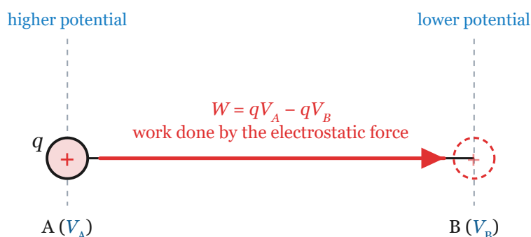
Figure 2-3-3 · The charge is released at the higher end of the ladder and arrives at the lower one. What it gives up in stored energy is exactly what the field has spent pushing it along, and only the height of the step between the two ends enters the sum.
