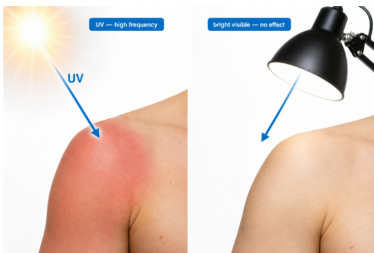
Figure 5-1-1 · An ordinary bright lamp leaves skin unharmed, while far weaker ultraviolet burns it — a clue that light's effect is set by its frequency (color), not its brightness.
