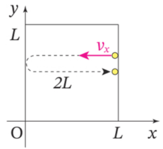
Figure 1-3-6 · Worked Example: between two hits on S the molecule covers a round trip of 2L , so it strikes S once every 2L/v_x .
