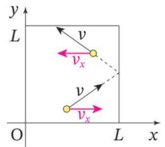
Figure 1-3-5 · Worked Example: a molecule crosses the box of side L and rebounds from the face at x = L , so v_x reverses while the speed v is unchanged.
