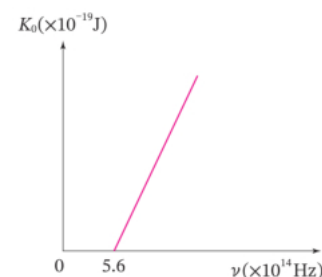
Figure 5-1-5 · Try: the photoelectrons' greatest energy plotted against the light frequency; the line meets the frequency axis at 5.6 \times 10^{14} \text{ Hz} .
