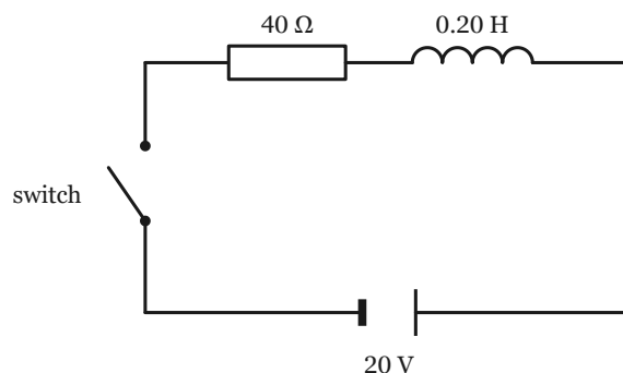
Figure 4-5-9 · A series loop of a 20 V battery, a 40 \Omega resistor, a 0.20 H coil, and a switch.
