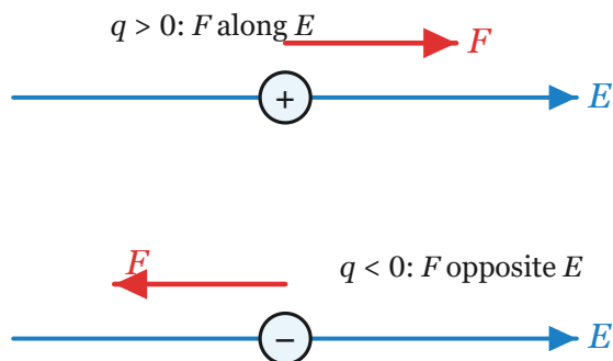
Figure 2-2-4 · In the same field E , a positive charge feels a force F along the field, while a negative charge feels a force along the same line but in the opposite direction.
