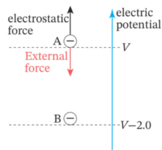
Figure 2-3-5 · Worked Example (c): a negative charge is carried slowly from A, at potential V , to B, at potential V - 2.0 V; the external force balances the electrostatic force.
