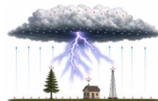
Figure 2-2-9 · Negative charge collects at a cloud's base and positive charge gathers on the ground; the field between them grows strong enough to break down the air, and a lightning discharge follows the path.
