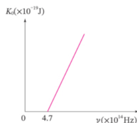
Figure 5-1-8 · Exercise: K_0 against \nu for the metal in this problem; the line meets the frequency axis at 4.7 \times 10^{14} Hz.
