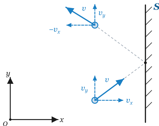
Figure 1-3-3 · Elastic collision at S : the perpendicular component reverses ( v_x \rightarrow -v_x ) while the parallel component v_y is unchanged, so the speed v is preserved.
