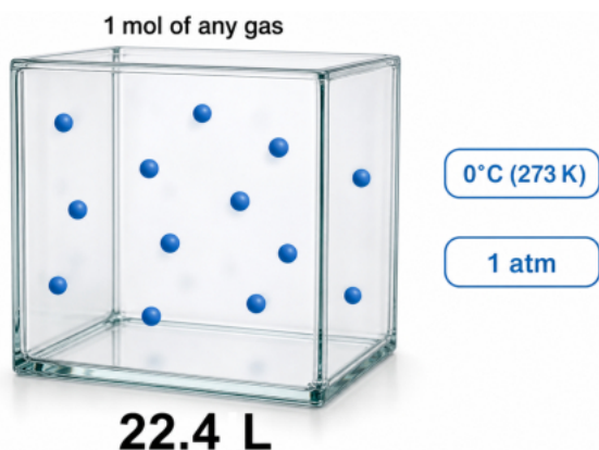
Figure 1-2-3 · One mole of any ideal gas fills 22.4 L in the standard state, 0°C and 1 atm.
