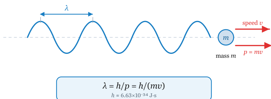
Figure 5-3-3 · The two descriptions drawn together: a lump of mass m traveling at speed v , and the wave that runs along the same path, its crest spacing fixed by the momentum.
