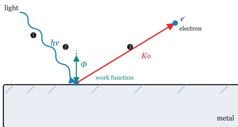
Figure 5-1-3 · The photon mechanism in three stages: ① one photon of energy h\nu is absorbed by a single electron; ② the electron pays the work function \Phi to escape the metal; ③ the remainder leaves as the maximum kinetic energy K_0 .
