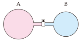
Figure 1-4-8 · Exercise 4: adiabatic containers A ( 0.62 \text{ m}^3 ) and B ( 0.21 \text{ m}^3 ) joined by a thin tube with a stopcock.
