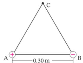
Figure 2-2-11 · Exercise 5: an equilateral triangle ABC of side 0.30 m with 4.0 \times 10^{-8} C at A and -4.0 \times 10^{-8} C at B.
