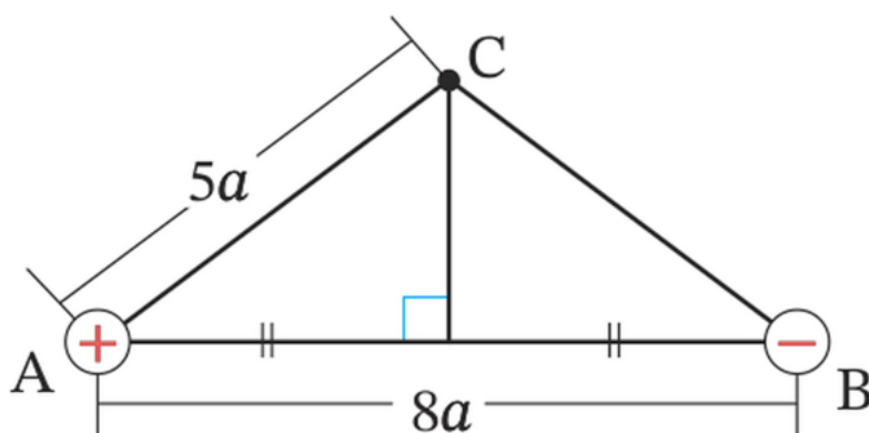
Figure 2-2-5 · Worked Example (b), from the original: the geometry alone — +q at A and -q at B a distance 8a apart, with C on the perpendicular bisector 5a from each.
