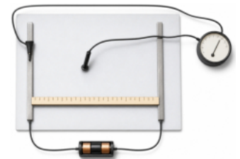
Figure 2-4-2 · Two straight parallel electrodes on conductive paper, a fixed distance d apart, are held at a steady voltage by a DC supply; the voltmeter keeps one probe on the negative electrode while the other reads the potential at each position x between them.
