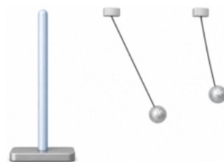
Figure 2-2-2 · A foil-covered ball on a thread, charged by touching the rod, serves as a small test charge of the same sign. Near the charged rod the thread swings far (a strong force); farther away it swings less — tracing the direction and strength of the field.
