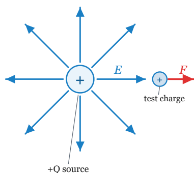
Figure 2-2-3 · The field of a positive point charge points radially outward. A unit positive test charge on a field line feels a force F in the same direction as the field E .
