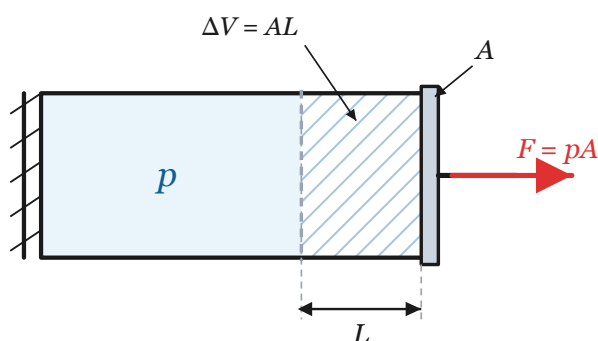
Figure 1-5-3 · At constant pressure p the gas pushes a piston of area A a distance L , doing work W = FL = pA \times L = p \Delta V on it.
