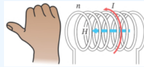
Figure 4-1-6 · Curl the fingers along the current I in the turns; the thumb points the way the field H runs along the axis.
