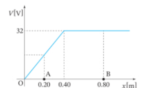
Figure 2-4-8 · Exercise 4: the potential rises uniformly to 32 V at x = 0.40 m and stays constant beyond it; A lies at x = 0.20 m and B at x = 0.80 m.
