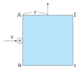
Figure 4-3-11 · Exercise 3: the particle crosses AB at a distance r from A, moving perpendicular to AB, and leaves across AD at the same distance r from A.
