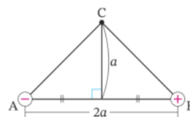
Figure 2-2-7 · Try 4: a point charge -q at A and +q at B, a distance 2a apart.
