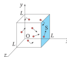
Figure 1-3-9 · Exercise: one mole of gas in a cubic container of side L , with the surface S perpendicular to the x -axis.
