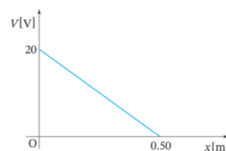
Figure 2-4-4 · Worked Example: the potential V falls uniformly from 20 V at x = 0 to 0 at x = 0.50 m.
