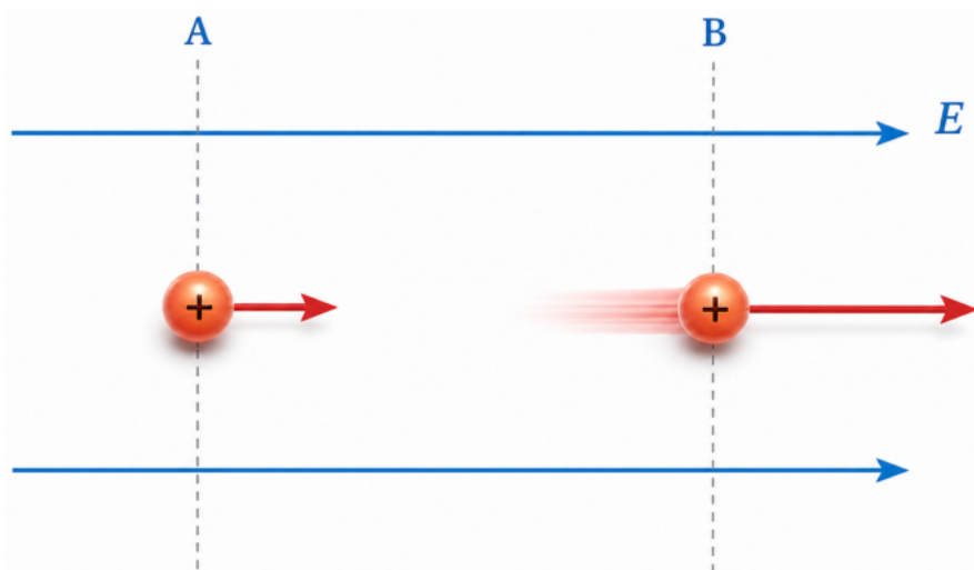
Figure 2-5-1 · A positive ion speeds up as it drifts from high potential A to lower potential B along the field E.
