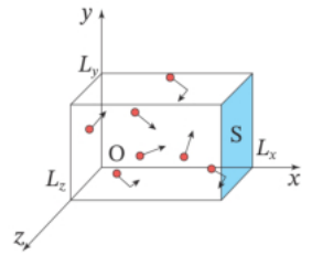
Figure 1-3-7 · Try 1: the same argument in a rectangular box of sides L_x, L_y, L_z , with the face S perpendicular to the x -axis.
