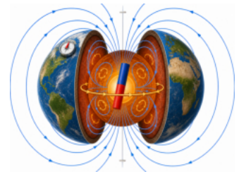
Figure 4-1-8 · The Earth as a giant electromagnet: a current in the convecting liquid-iron core builds a dipole field, and a surface compass lines up with it.
