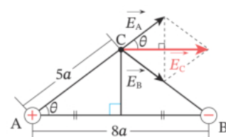
Figure 2-2-6 · Worked Example: at C the field of the positive charge at A and that of the negative charge at B are equal in size, so their vertical parts cancel and the resultant E_C lies parallel to AB.
