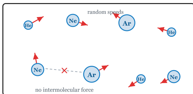
Figure 1-4-3 · Monatomic molecules — single atoms of He, Ne, and Ar — moving in random directions at random speeds inside a box, with no intermolecular force acting between them.
