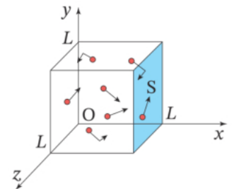
Figure 1-3-4 · Worked Example: molecules move in a cube of side L ; each collision with the shaded wall S reverses the x -component of a molecule's momentum.
