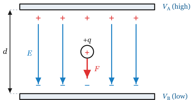
Figure 2-4-3 · A uniform field E between two horizontal plates a distance d apart runs from the high-potential plate V_A to the low-potential plate V_B ; a positive charge +q in the gap feels a force F = qE from high toward low potential.
