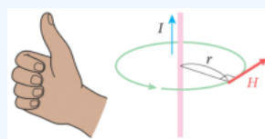
Figure 4-1-4 · Grip the wire so the thumb points along the current I ; the fingers curl the way the field H circles it.
