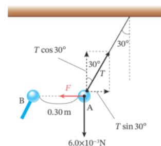
Figure 2-1-5 · Worked Example: the forces on A resolved — the tension T with its components T \cos 30^\circ and T \sin 30^\circ , the electrostatic force F , and the weight 6.0 \times 10^{-3} \text{ N} .
