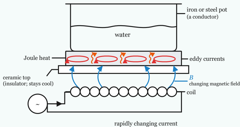
Figure 4-4-9 · Inside an IH cooking heater. A rapidly changing current in the coil under the ceramic top sends a changing magnetic field up through it and into the base of the pot. Because that base conducts, the changing flux drives eddy currents round inside the metal, and their Joule heating warms the pot itself — the ceramic top stays cool.
