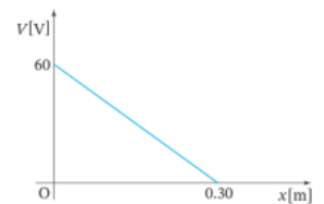
Figure 2-4-7 · Exercise 3: the potential V falls uniformly from 60 V at x = 0 to 0 at x = 0.30 m.
