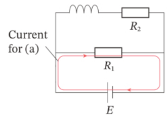
Figure 4-5-5 · Worked Example (a): immediately after the switch closes the coil branch carries nothing, so the whole circulation is the loop drawn in red — battery, R_1 , and back.
