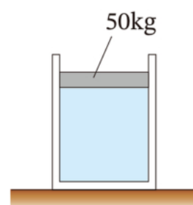
Figure 1-1-7 · Try 1: air enclosed in a cylinder by a smoothly moving piston of cross-sectional area 4.9 \times 10^{-2}\text{ m}^2 and mass 50 kg.
