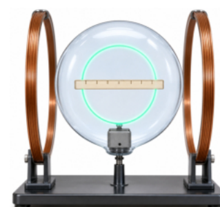
Figure 4-3-2 · A fine-beam (e/m) tube: an electron gun fires a beam that a coil field bends into a glowing circle, whose diameter 2r is read off a ruler across the tube.
