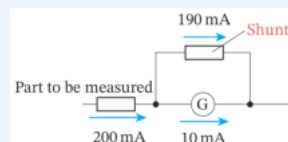
Figure 3-1-4 · Shunt wiring, imported from the original: the meter dial and a low resistance bridge one and the same pair of junctions, so the line arriving from the left divides between the two branches and reunites on the right. The arrow labels give the division for the Example beside it.
