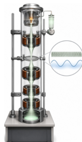
Figure 5-3-5 · An electron-microscope column focuses the electron beam with magnetic lenses onto the specimen; the inset compares the very short electron wavelength (green) with the far longer wavelength of light (blue) — that is why the electron beam resolves fine detail light cannot.
