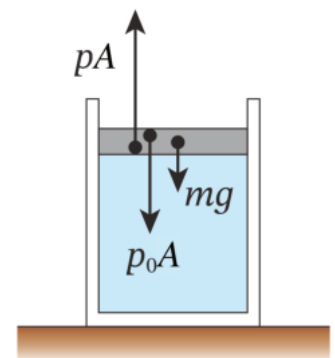
Figure 1-1-5 · Worked Example (a): the balance of forces on the piston — the gas pushes up with pA , while atmospheric p_0A and the weight mg push down.
