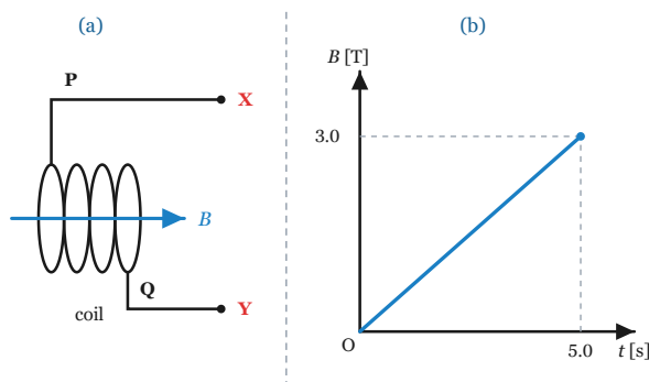
Figure 4-4-4 · (a) The coil with terminals P and Q, external points X and Y, and the reference arrow B that fixes the positive field direction. (b) The flux density B rises steadily from 0 to 3.0 T at t = 5.0 s.
