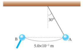
Figure 2-1-9 · Exercise 2: ball A of mass 2.0 \times 10^{-3} kg hangs beside ball B carrying 4.9 \times 10^{-7} C, both at the same height.
