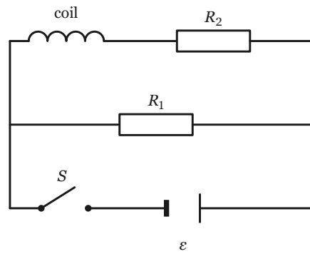
Figure 4-5-4 · Battery of emf \varepsilon ; resistor R_1 sits directly across the battery, while resistor R_2 in series with the coil forms a second branch; switch S in the supply line.
