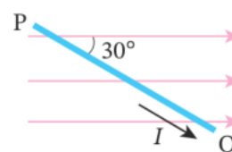
Figure 4-2-8 · Exercise 5: the conducting rod PQ lies at 30^\circ to a uniform magnetic field directed to the right, with the current I flowing from P to Q.
