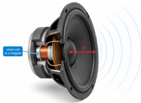
Figure 4-2-1 · A loudspeaker's voice coil hangs in a magnet's field: the music current through the coil makes the field push it — and the cone glued to it — in and out (force F_B ), so a larger current gives a bigger push.
