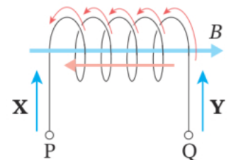
Figure 4-4-5 · Worked Example (b): the induced current in the coil, drawn in red, sets up a field opposing the growth of B , so the current in the outside circuit runs toward Y.
