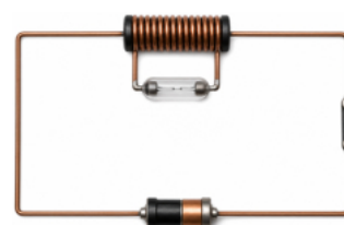
Figure 4-5-2 · A neon lamp is wired across the coil; with a steady current the lamp stays dark, since the small battery voltage is far below its striking voltage.
