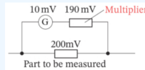
Figure 3-1-5 · Multiplier wiring, imported from the original: dial and resistor lie one behind the other along a single branch, itself bridged across the component under test, so one current threads both and the labels show how the applied 200 mV is shared out.
