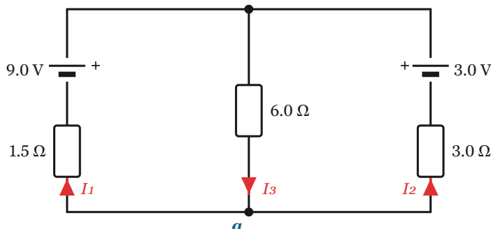
Figure 3-2-7 · Try: batteries 9.0 V and 3.0 V with resistors 1.5\ \Omega , 6.0\ \Omega , and 3.0\ \Omega in a two-loop network — the 9.0 V battery shares its branch with the 1.5\ \Omega resistor, the 3.0 V battery with the 3.0\ \Omega resistor, and the 6.0\ \Omega resistor is the shared middle branch.
