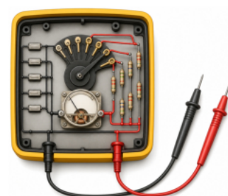
Figure 3-1-8 · A single central meter movement is reused for every range, with short thick low-resistance shunts wired in parallel for current ranges and long thin high-resistance multipliers wired in series for voltage ranges, one at a time selected by the rotary switch.
