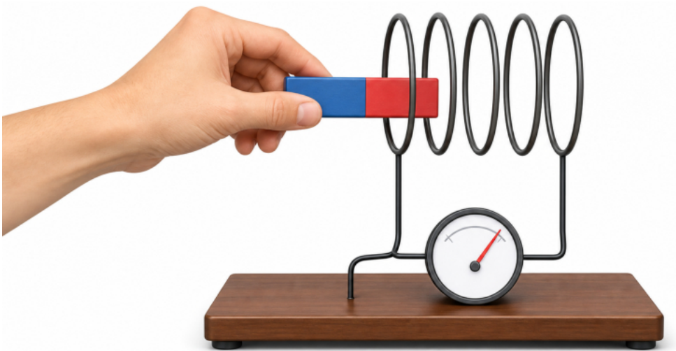
Figure 4-4-1 · A coil joined only to a galvanometer, with no battery; moving the bar magnet along the coil axis swings the needle while the field through the coil changes.
