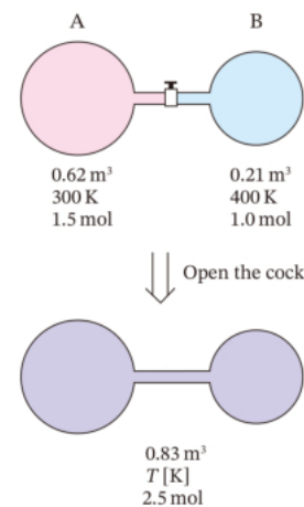
Figure 1-4-5 · Worked Example: the two containers before the stopcock is opened ( 0.62 \text{ m}^3 , 300 \text{ K} , 1.5 \text{ mol} and 0.21 \text{ m}^3 , 400 \text{ K} , 1.0 \text{ mol} ) and the combined gas afterwards ( 0.83 \text{ m}^3 , T , 2.5 \text{ mol} ).
