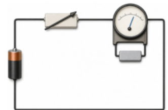
Figure 3-1-2 · Bench setup: a milliammeter in series with a supply and a rheostat, with a small resistor wired directly across the meter terminals so part of the line current bypasses the movement.
