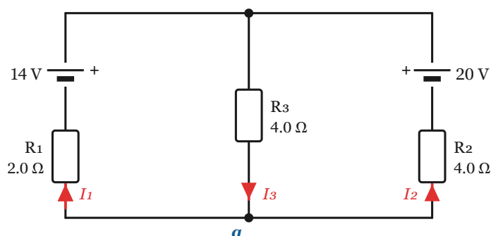
Figure 3-2-11 · Exercise 3: batteries 14 V and 20 V with R_1 = 2.0 \Omega , R_2 = 4.0 \Omega , R_3 = 4.0 \Omega in a two-loop network — the 14 V battery shares its branch with R_1 , the 20 V battery with R_2 , and R_3 is the shared middle branch.
