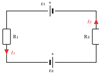
Figure 3-2-5 · Kirchhoff's second law around a closed loop with two sources and two resistors: \varepsilon_1 + \varepsilon_2 = R_1 I_1 + R_2 I_2 .
