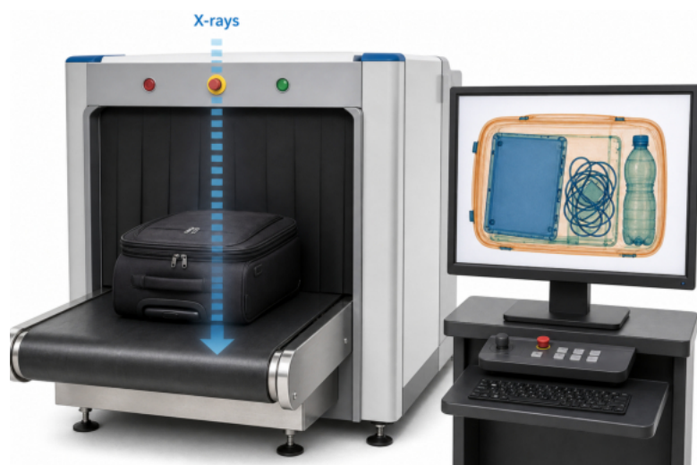
Figure 5-2-1 · An airport scanner makes X-rays by driving accelerated electrons into a metal target; the rays pass through the bag to image its contents.
