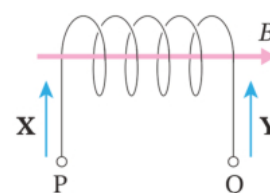
Figure 4-4-10 · Exercise 3: the coil with terminals P and Q, the reference arrow B , and the senses X and Y in the outside circuit.
