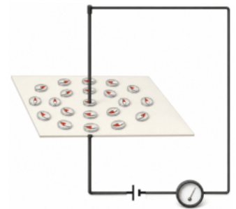
Figure 4-1-2 · A vertical wire through a card: small compasses line up on circles around the wire, mapping the field while the ammeter reads the current I .
