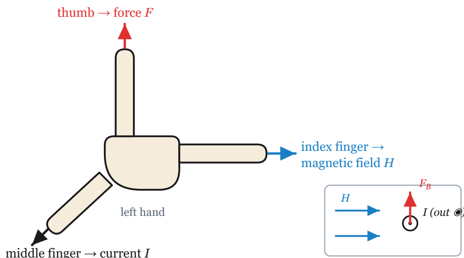
Figure 4-2-3 · Fleming's left-hand rule: with the thumb, index finger, and middle finger held at right angles, the middle finger points along the current I , the index finger along the magnetic field H , and the thumb gives the force F_B — as in the inset rod carrying current out of the page across a rightward field.
