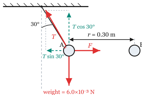
Figure 2-1-3 · Free-body diagram of ball A: the string deflects 30^\circ from the vertical toward B (0.30 m away), so the tension T (with components T \cos 30^\circ up and T \sin 30^\circ across), the electrostatic force F toward B, and the weight 6.0 \times 10^{-3} N balance.
