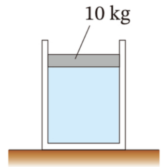
Figure 1-1-4 · Worked Example (a): air enclosed in a cylinder by a smoothly moving piston of mass 10 kg.
