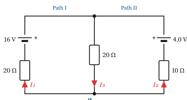
Figure 3-2-6 · Worked Example: two batteries ( 16 \text{ V} , 4.0 \text{ V} ) and three resistors ( 20 \Omega , 20 \Omega , 10 \Omega ) form two loops sharing a middle branch that meet at junction a; assumed currents I_1 , I_2 , I_3 .
