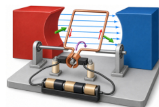
Figure 4-2-7 · A simple DC motor: current I in a coil between the N and S poles feels opposite forces F_B = IBL on its two sides, which turn the coil; a commutator reverses the current each half-turn so the rotation keeps going the same way.
