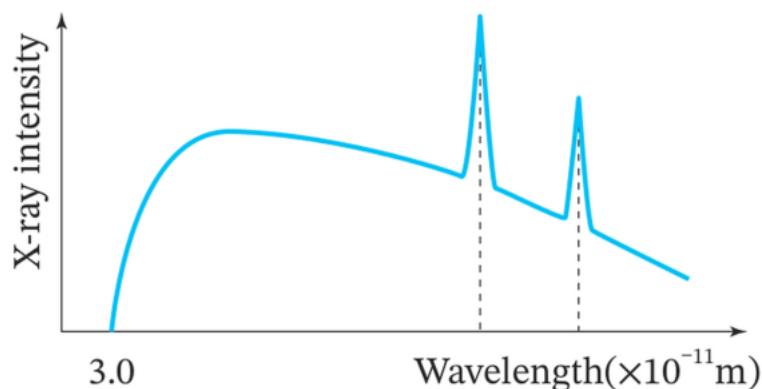
Figure 5-2-5 · Exercise 2: the intensity–wavelength spectrum of the X-rays, with a sharp cut-off at 3.0 \times 10^{-11} m and two characteristic peaks.
