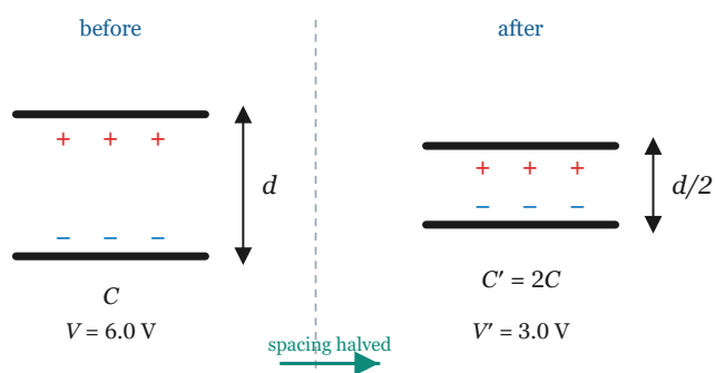
Figure 2-6-5 · The same capacitor before and after the spacing is halved: the gap becomes d/2 and the capacitance doubles to C' = 2C . Drawn for part (a), with the battery disconnected: the charge on the plates is unchanged, so the potential difference halves to 3.0 V.
