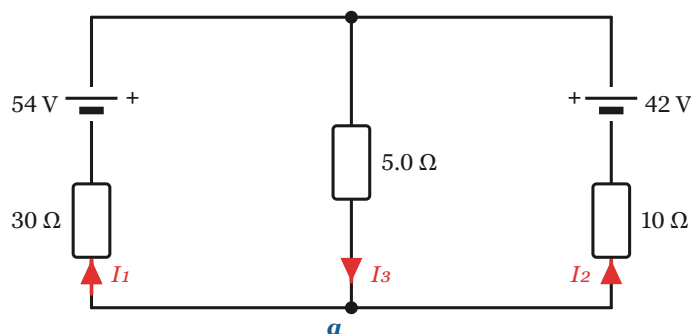
Figure 3-2-9 · Exercise 1: batteries 54 V and 42 V with resistors 30 \Omega , 5.0 \Omega , and 10 \Omega in a two-loop network.
