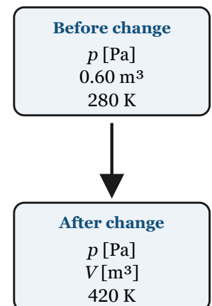
Figure 1-1-6 · Worked Example (c): the gas before and after being heated at constant pressure.
