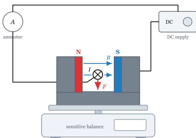
Figure 4-2-2 · A conducting rod of length L carrying current I rests between the poles of a magnet on a sensitive balance, which reads the force. A variable DC supply and an ammeter set and measure I . The rod runs into the page, at right angles to B , so the force on it is vertical and the balance reads it.
