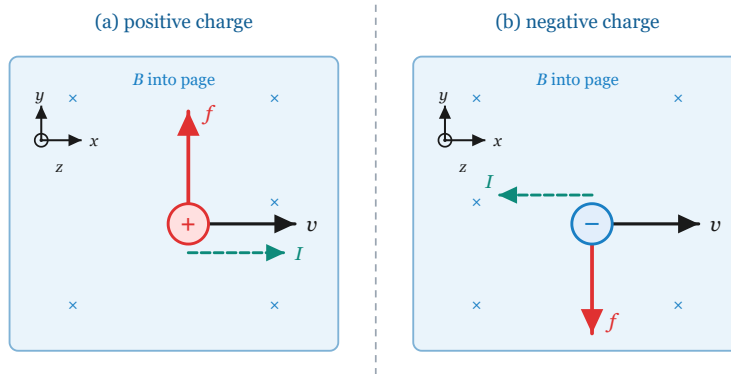
Figure 4-3-3 · Lorentz force in a field into the page: for a positive charge the equivalent current I runs along v and f points up; for a negative charge I runs opposite v and f points down.
