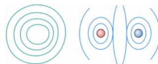
Figure 2-3-7 · Contour lines on a hill and equipotential lines around two charges obey the same rule: where the lines crowd together, the slope is steep and the field is strong.
