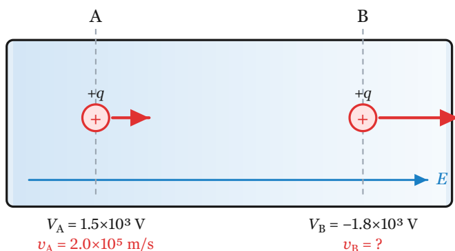
Figure 2-5-4 · The positive ion passes A with a short velocity arrow ( v_A = 2.0 \times 10^5 \text{ m/s} , V_A = 1.5 \times 10^3 \text{ V} ) and B with a longer one ( V_B = -1.8 \times 10^3 \text{ V} , v_B = ? ).
