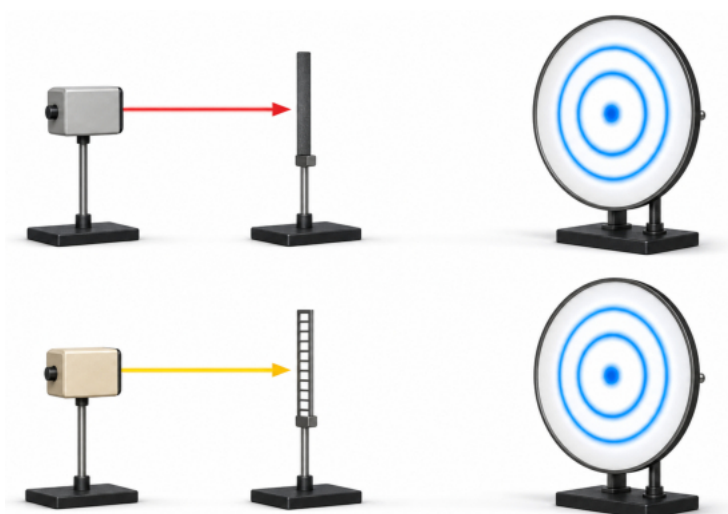
Figure 5-3-1 · An electron beam through a graphite film makes the same concentric diffraction rings that light makes through a grating — the electron beam travels as a wave.
