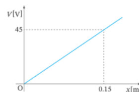
Figure 2-4-5 · Try: the potential V rises uniformly with x , reaching 45 V at x = 0.15 m.
