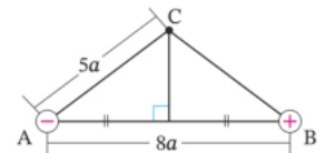
Figure 2-2-12 · Exercise 6: a charge -q at A and +q at B a distance 8a apart, with C off the line joining them.
