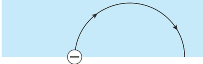
Figure 4-3-4 · Worked Example: an electron enters a uniform field B perpendicular to the page and describes a semicircle inside it.
