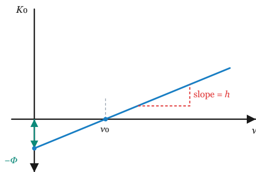
Figure 5-1-4 · Maximum kinetic energy K_0 against frequency \nu : a straight line of slope h that meets the K_0 -axis at the intercept -\Phi and crosses the \nu -axis at the threshold frequency \nu_0 .
