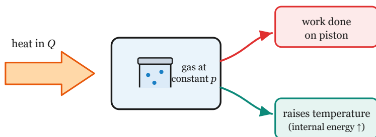
Figure 1-6-3 · At constant pressure the incoming heat Q splits: part raises the internal energy (temperature), part does work on the rising piston.
