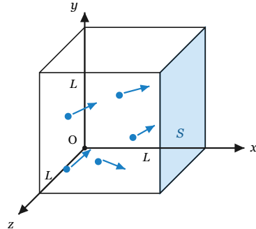
Figure 1-3-2 · Cubic container of side L with axes x, y, z and the shaded face S \perp x ; gas molecules move along the velocity arrows.
