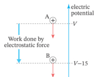
Figure 2-3-4 · Worked Example (b): a positive charge falls from A at potential V to B at V - 15 , and the electrostatic force does the work.
