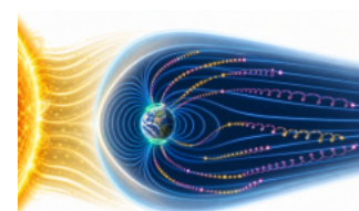
Figure 4-3-8 · Solar-wind particles are captured by Earth's magnetic field and spiral along the field lines toward the poles, where they light the atmosphere as an aurora.
