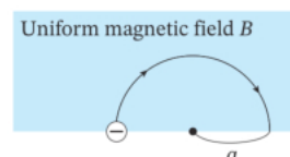
Figure 4-3-10 · Exercise 2: the electron enters the uniform field B and turns through a semicircle of radius a .
