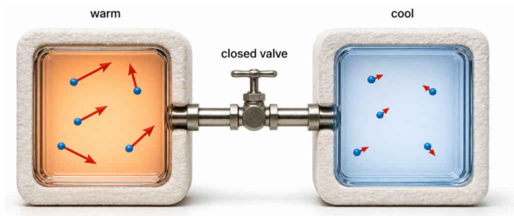
Figure 1-4-1 · Two insulated flasks of helium, one warm and one cool, joined by a closed valve; the warmer atoms move faster.
