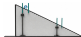
Figure 2-5-2 · A marble released at height h_A (point A) slides down the smooth, low-friction ramp to the lower point B at height h_B ; a photogate reads its speed at each point.
