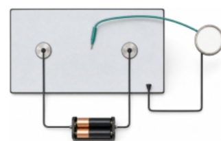
Figure 2-3-2 · Two electrodes on conductive paper are wired to a battery; a voltmeter keeps one probe on a fixed reference while the other is moved over the sheet to find points of equal potential.
