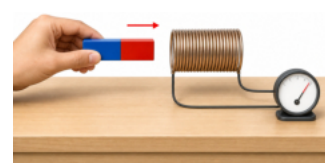
Figure 4-4-2 · Bench setup: a many-turn coil is wired to a center-zero galvanometer; the bar magnet is inserted into and withdrawn from the coil along its axis.
