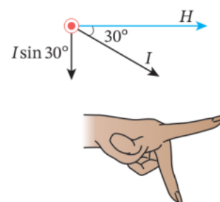
Figure 4-2-5 · Worked Example: the current I crosses the field H at 30^\circ , so only the perpendicular component I \sin 30^\circ drives the force; the hand shows Fleming's left-hand rule.
