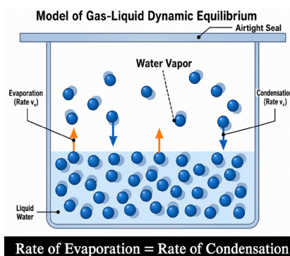
Fig 1.2.1 the relation between rate of evaporation and rate of condensation
