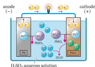
Figure 2.4.1 Lead–acid battery
