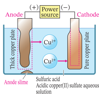
Figure 2.6.2. Electrolytic Refining of Copper
