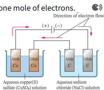
Figure 2.6.1 Electrolysis using two electrolytic cells
