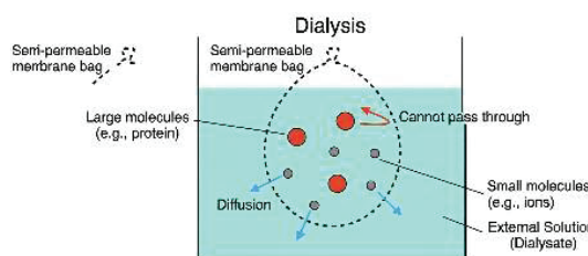
Figure 1.11.1 Dialysis Property
