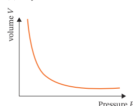
Fig 1.4.1 Boyle's Law
