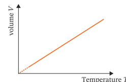
Figure 1.4.2 Charles's law
